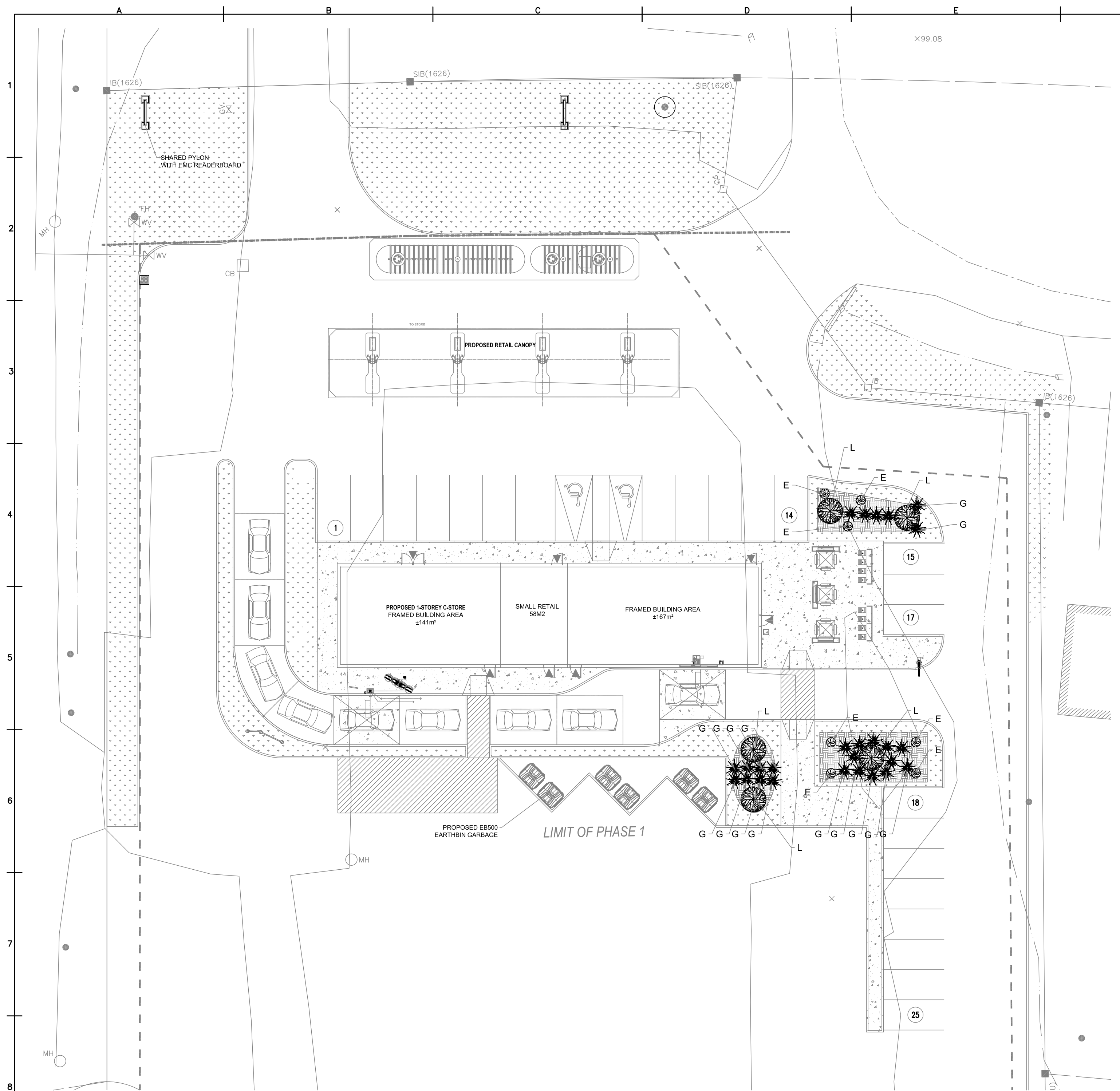
1 LANDSCAPE PLAN 1:300
